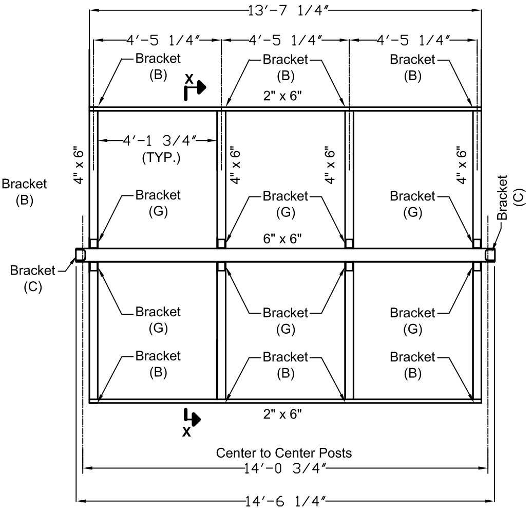
PLAN AT TRACK BEAMS
