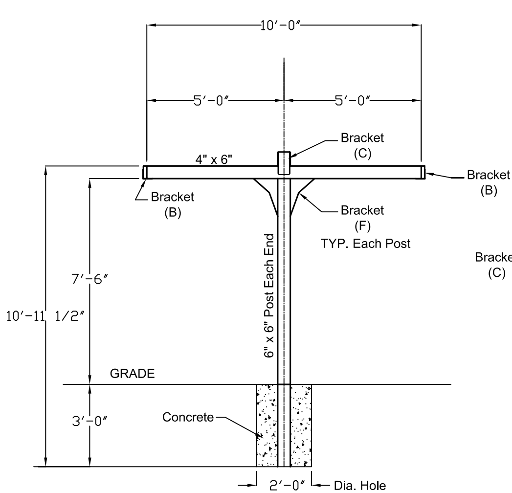
END VIEW
